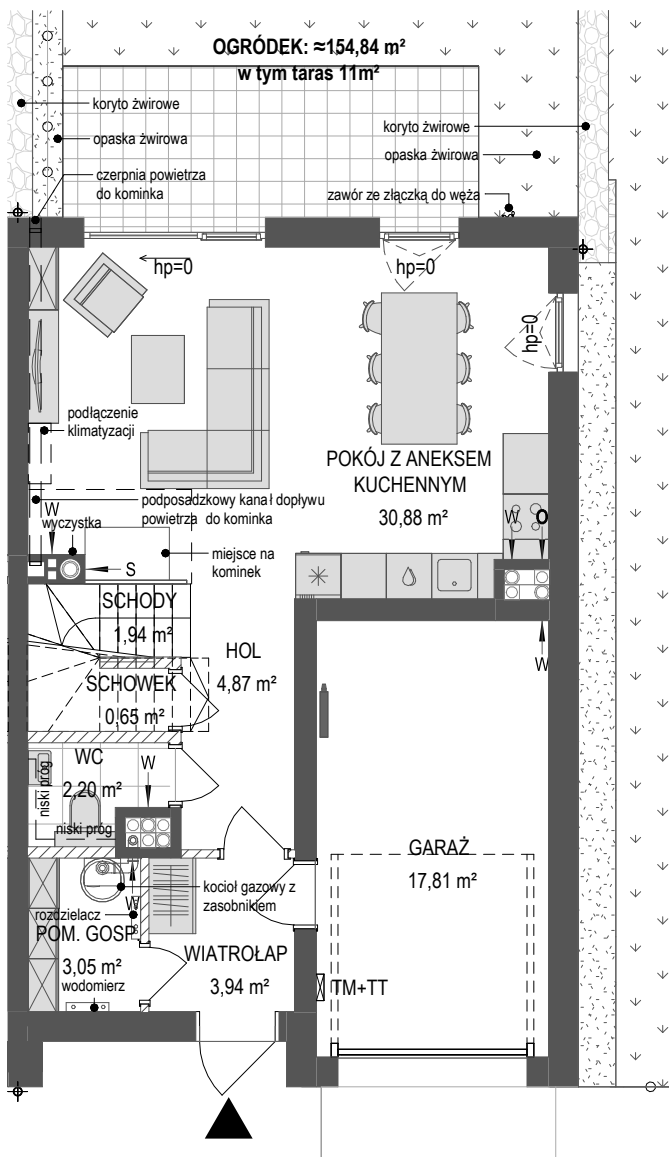
PARTER 65,34 m 2
